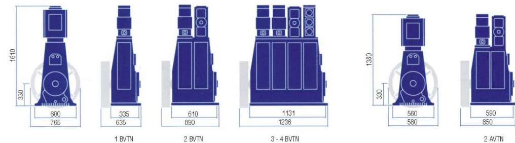
BVTN Compressor
